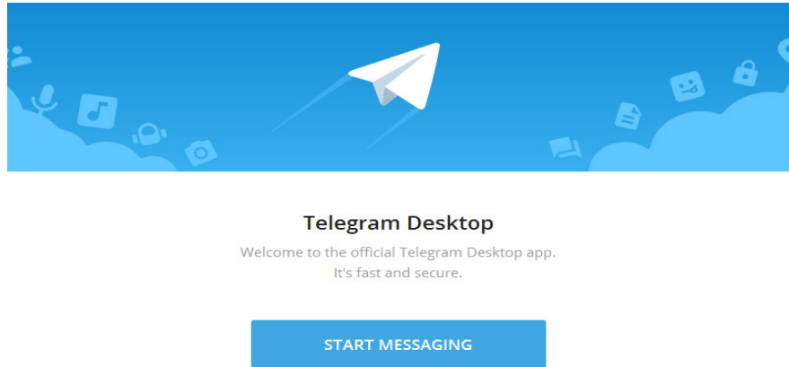
Figure 4.9 Telegram
