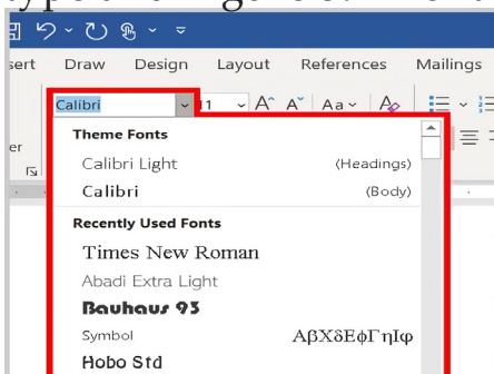
Figure 3.13. Font type
